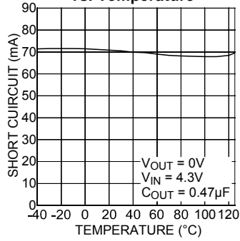
Short Circuit Current vs. Temperature
