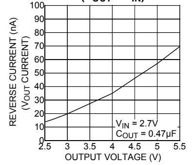
Reverse Leakage Current (VOUT > VIN)
